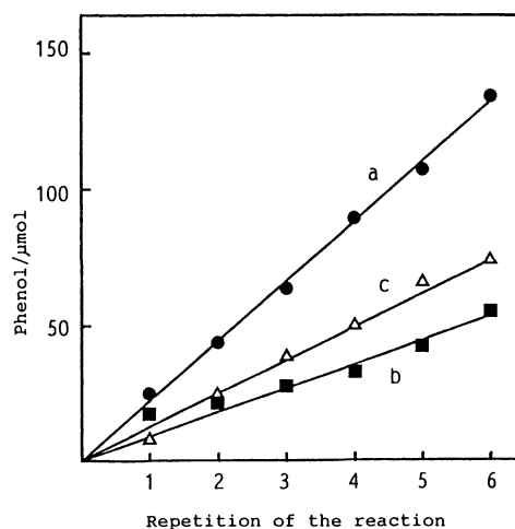
Fig. 2. Effect of preparation methods on the catalyst performance. The reactions were carried out in the same manner as described in Table 3 except that hydrogen reduction (30 min) and air-oxidation (30 min) were applied in each reaction cycle. Symbols stand for the catalysts of type A (●), B (■), and C (△), respectively.
